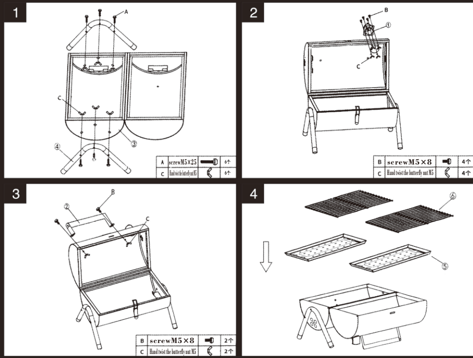
Installation completion diagram
